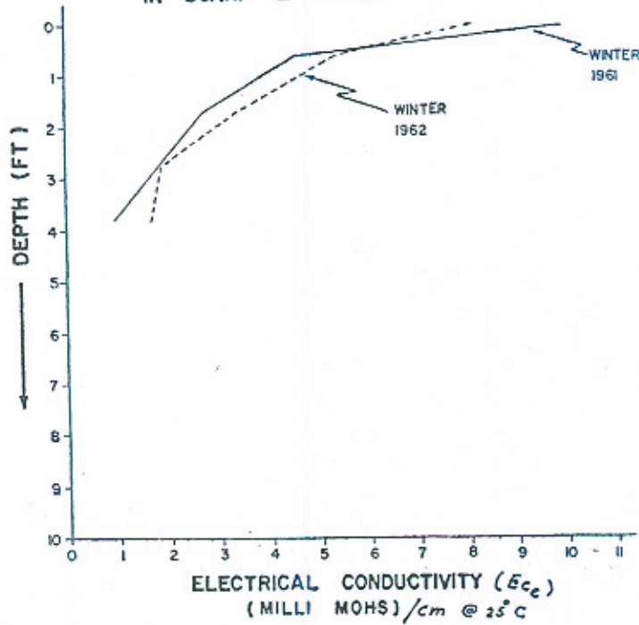
CHANGES IN E_c OF SOIL PROFILE FOR FINE-TEXTURED SOIL AVERAGE FOR 8 TEST PLOTS IN SCARP I AREA
