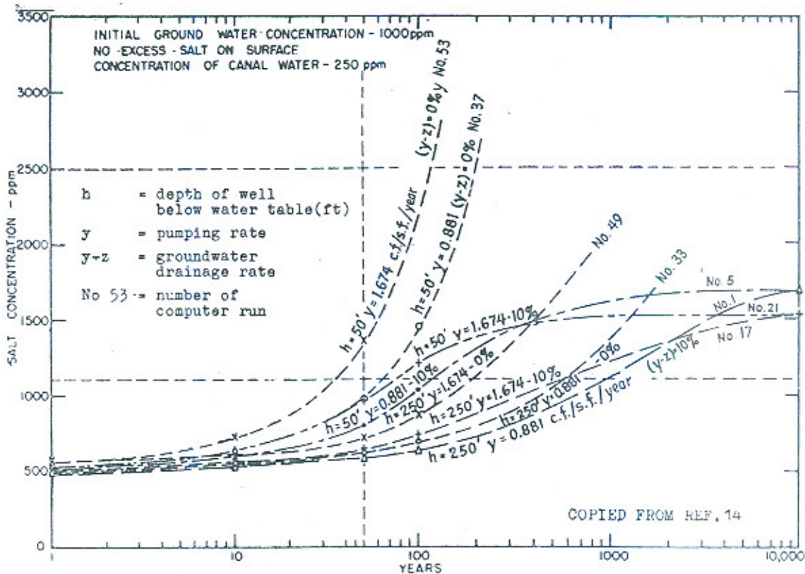
FIG. 3 SALT CONCENTRATION OF APPLIED IRRIGATION WATER
