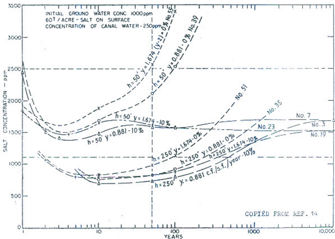
FIG. 4 SALT CONCENTRATION OF APPLIED IRRIGATION WATER
